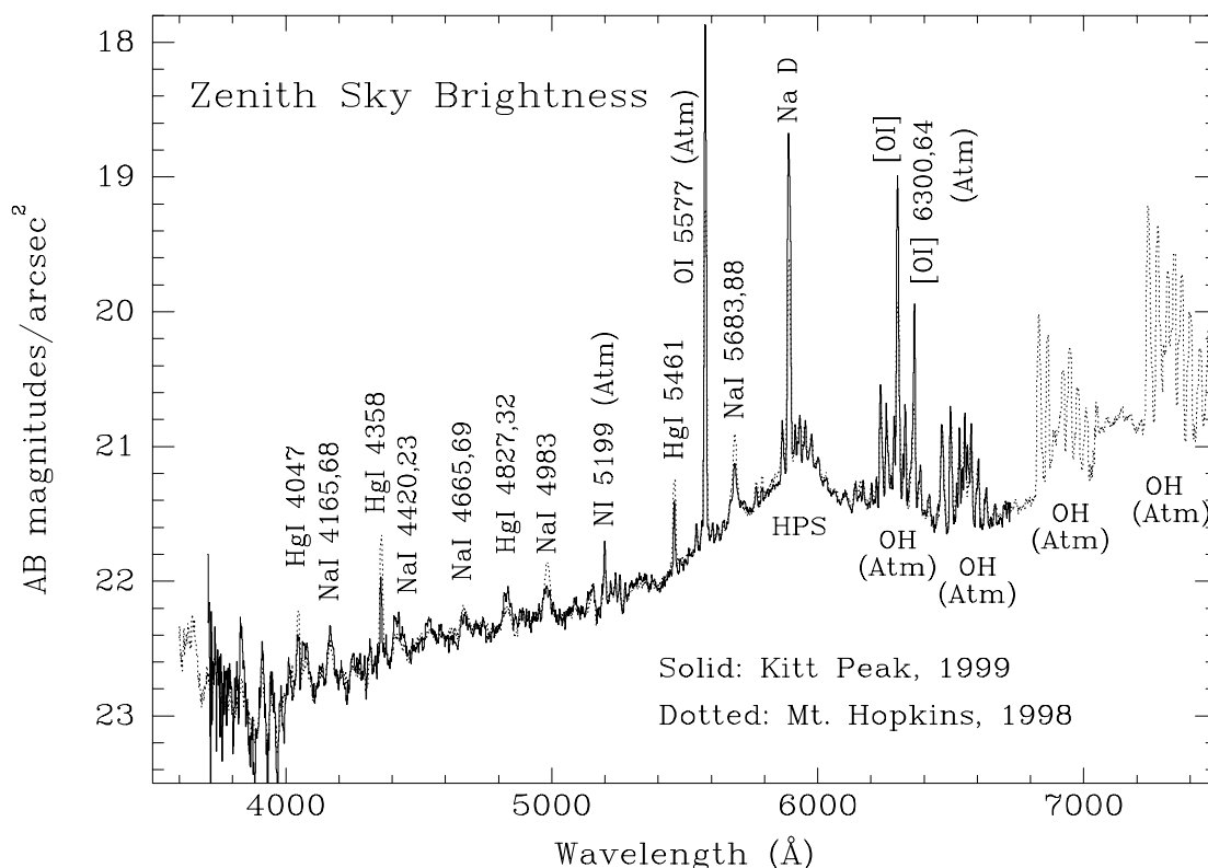
FIG. 1.—Second-epoch observations of the spectrum of the night sky at the zenith above Kitt Peak (solid line) and Mount Hopkins (dashed line). Emission features from natural and man-made sources are marked. High-pressure sodium (HPS) lamps are responsible for the broad feature extending from \sim 5500 to 6500 \text{ \AA} .
